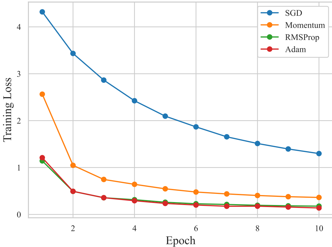
Plot 6: Training Loss vs. Epoch (Optimizers)
